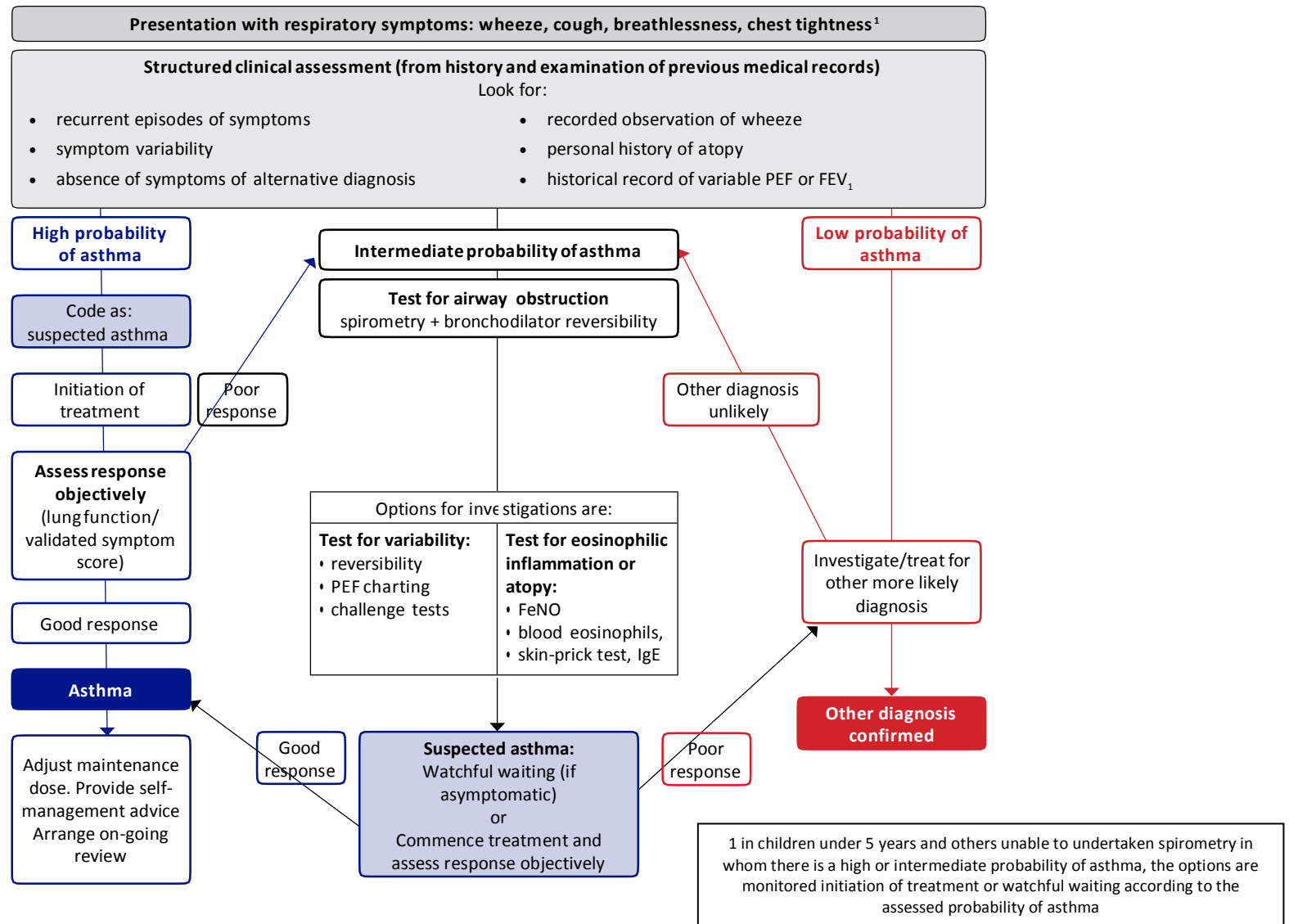
Figure 1: Diagnostic algorithm
